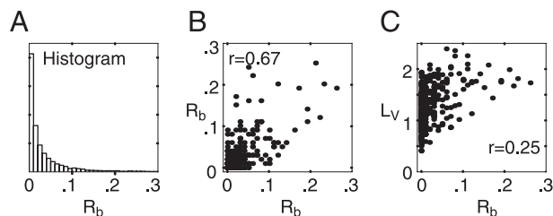
FIG. 8. A : histogram of the rates of bursts R_b for all recorded sequences of 100 ISIs. Although the data ranged from 0 to 0.67, the number of 100 ISI sequences of R_b > 0.3 was very small (114 out of 8526, 1.3%) and is not pictured here. B : scattergram of R_b for 2 sequences of 100 ISIs in different time periods, each sampled from the same neuron. C : scattergram of R_b – L_v for the same sequences of 100 ISIs individually sampled from the 288 neurons.
