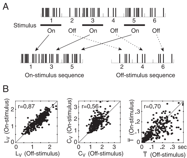
FIG. 5. A : schema for concatenating spike sequences of stimulus periods and interstimulus periods, respectively, to construct stimulus-present and stimulus-absent spike sequences. B : scattergrams of the local variation L_v (left), the coefficient of variation C_v (center), and the mean interspike interval \bar{T} (right), for 2 sequences of 100 ISIs from the stimulus-present and stimulus-absent spike sequences, each derived from the same neuron.
