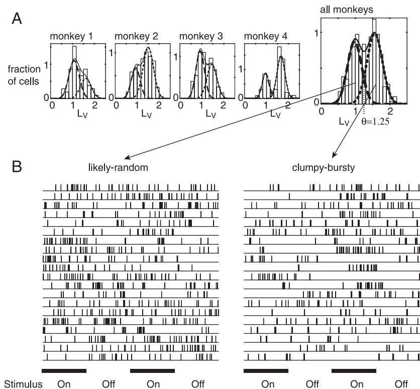
FIG. 3. A : 2-component Gaussian distributions fitted to the set of L_v values for monkeys 1–4 and the summed data for all the monkeys. Original data were plotted as histograms, fitted 2 Gaussian distributions were depicted as dotted lines, and the sum of the 2 Gaussian distributions was depicted as a solid line. B : sample raster diagrams of 20 "likely random" firing neurons of 0.6 < L_v < 1.1 and 20 "clumpy-bursty" firing neurons of 1.3 < L_v < 1.9 . Each vertical bar indicates time of occurrence of a spike. Each raster contains 20–50 spikes. Clumpy-bursty rasters appear to have considerably fewer than the real number of spikes because the spikes clump together in time.
