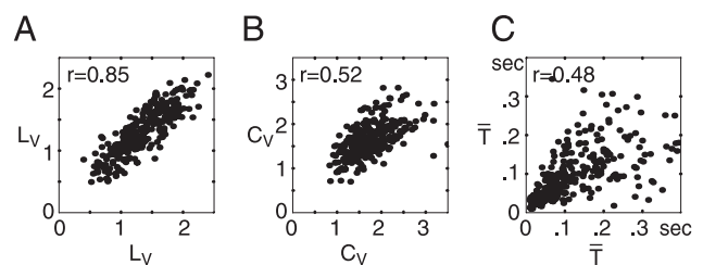
FIG. 4. Scattergrams of the local variation L_v ( A ), the coefficient of variation C_v ( B ), and the mean interspike interval \bar{T} ( C ), for 2 sequences of 100 ISIs from different time periods, each sampled from the same neuron. Each dot denotes data from a single neuron. n = 288 .
