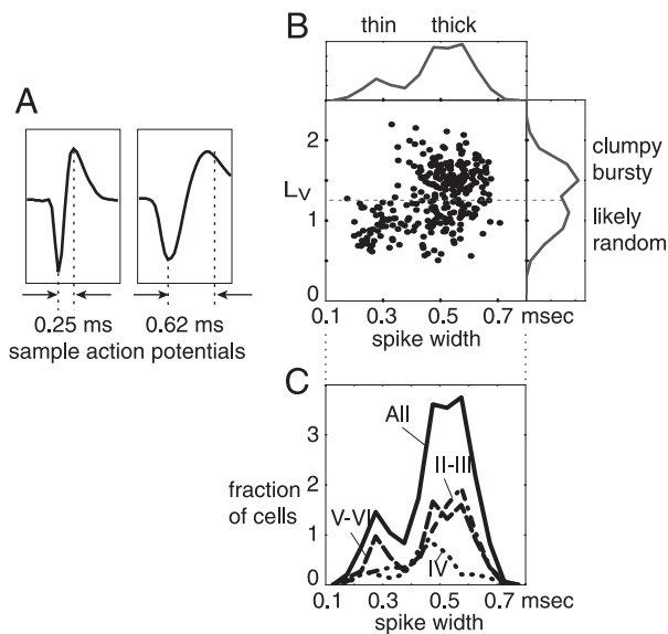
FIG. 9. A: 2 examples of spike shapes with short and long widths. B: distribution of the spike widths and the L_v values of the 288 neurons. C: distributions of the spike widths from all layers, layers II–III, layer IV, and layers V–VI, depicted as solid, dot-dashed, dotted, and dashed lines, respectively.
