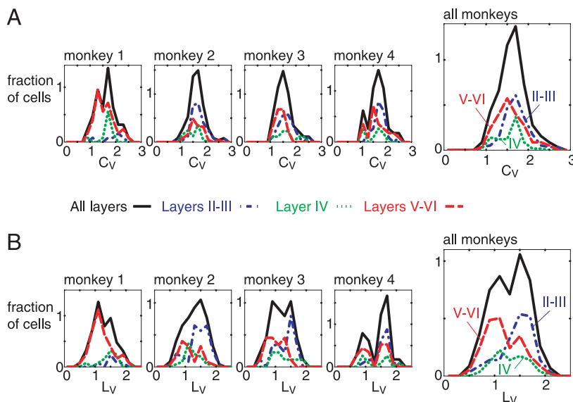
FIG. 2. Distributions of C_V (A) and L_V (B) values for area TE of monkeys 1–4 and the summed data for all monkeys. “Fraction of cells” is the number of cells counted in each bin of width \Delta = 0.2 , divided by the total number of cells and \Delta ( =0.2 ). Data from all layers, layers II–III, layer IV, and layers V–VI are depicted as black solid, blue dot-dashed, green dotted, and red dashed lines, respectively.
