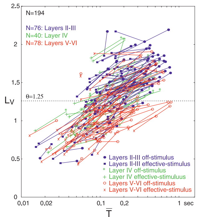
FIG. 6. Scatter plot of L_v and \bar{T} for effective-stimulus periods and interstimulus periods. Each line shows data from each of the 194 neurons analyzed. Blue lines indicate data from layer II–III neurons, green lines those from layer IV neurons, and red lines those from layer V–VI neurons.
