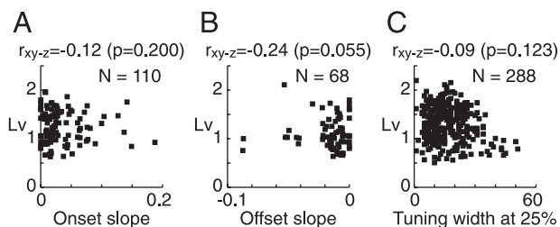
FIG. 7. A : relationship between L_v and the slope of response onset. Three points with a large slope are not included in the graph. B : relationship between L_v and the slope of response offset. See text for definition of the slope of response onset and offset. C : relationship between L_v and the number of stimuli that evoked responses >25\% of the maximal response. Correlation coefficient or partial correlation coefficient is provided as r or r_{xy-z} with corresponding P values.
