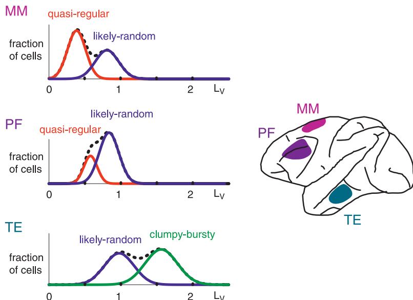
FIG. 10. Various types of spike sequences categorized according to L_V values. Centers of the fitted 2-component Gaussian distributions of L_V for the medial motor areas MM, the prefrontal cortex PF, and area TE of the inferior temporal cortex are located at {0.8 (likely random), 0.4 (quasi-regular)}, {0.8 (likely random), 0.6 (quasi-regular)}, and {1.6 (clumpy-bursty), 1.0 (likely random)}, respectively. Data for MM and PF are from Shinomoto et al. (2003).
